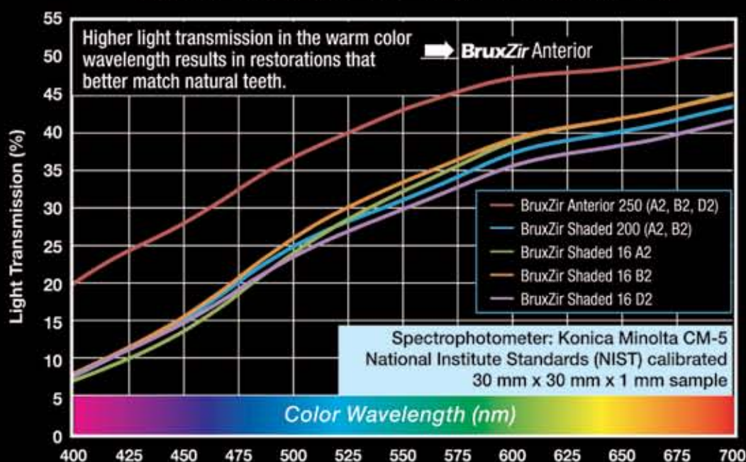
Light Transmission vs. Wavelength 1.0 mm Thickness
