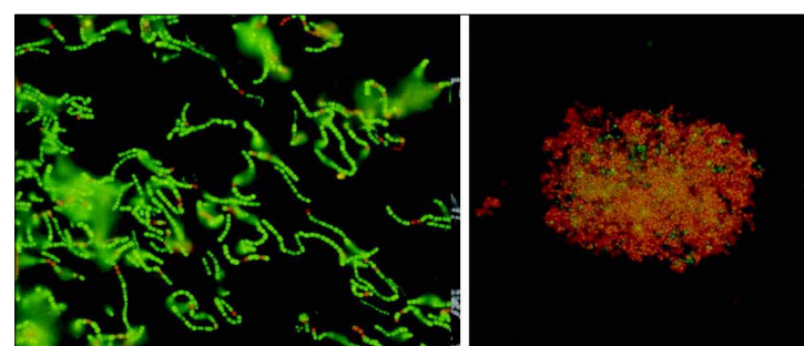
Figure 2. Bactericidal activity assessment 16 hours after exposure. Left; water control. Right; stannous fluoride/sodium hexametaphosphate dentifrice. Green-stained cells are live microbial cells; red-stained cells are dead cells (from Ramji et al 21 ).
