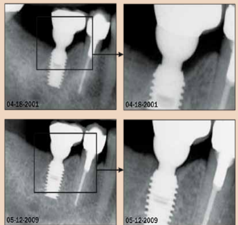
Fig 3 Periapical radiographs of a 5 x 8-mm HA-coated Bicon implant in the mandibular right posterior area restored with a metal-ceramic crown cemented to a titanium prefabricated abutment. Note the crestal bone gain between crown insertion (2001) and the last recall appointment (2009); the bone has grown coronal to the implant-abutment interface and toward the spherical base of the abutment. This patient used daily doses of celecoxib or ibuprofen to control arthritic pain.
