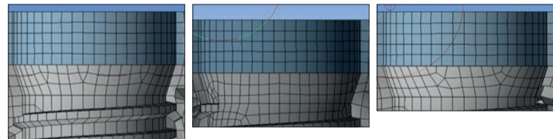
Fig. 6 - Meshing process, (a) mesh of universal prosthesis, (b) mesh of locator prosthesis, (c) mesh of Equator prosthesis.
