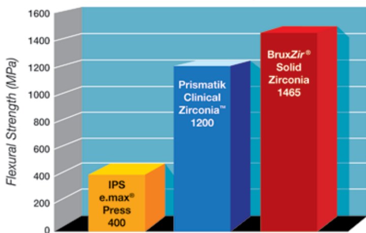
Flexural Strength 1
