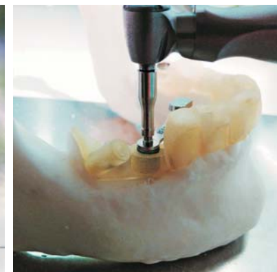
Fig. 5: Drill attached to the extension passing through the reduction sleeve. The extension allows the drill to be guided correctly without touching the template on the adjacent tooth with the contra-angle handpiece.
