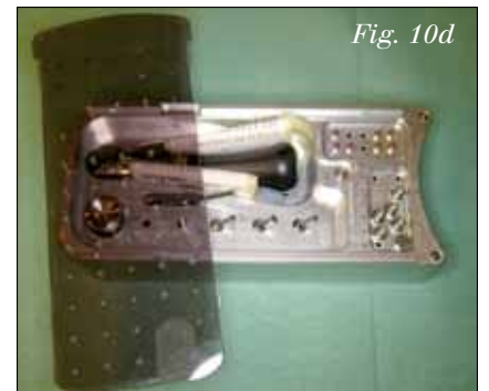
Figs. 10a–d: Preparation of the work rack and removal of the blades.
