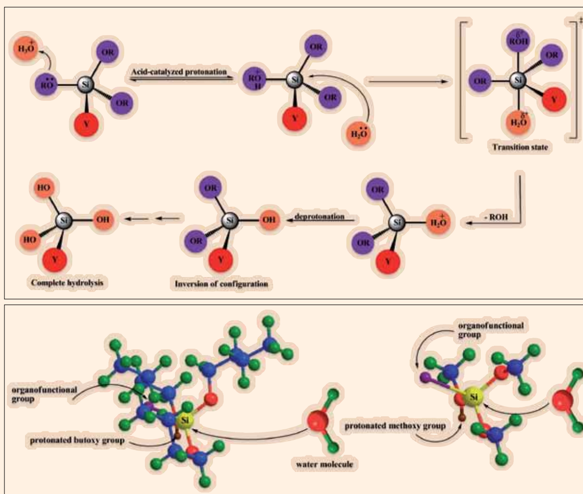
Fig. 1: The silane hydrolysis mechanism.— Fig. 2: The steric effect of alkoxy groups on silane hydrolysis using ball-and-stick models between butoxysilane and methoxysilane.
