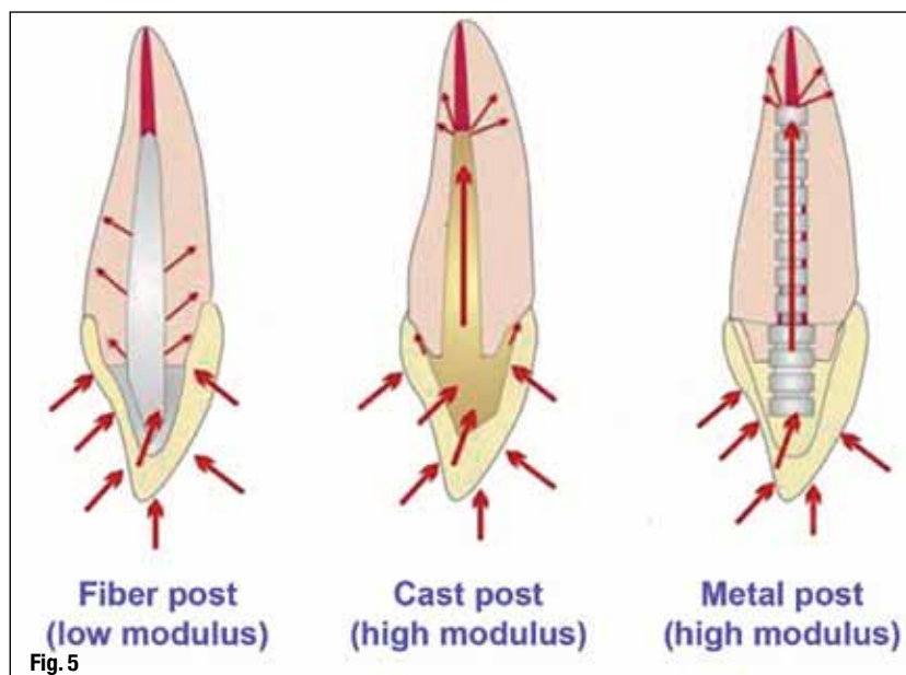
Fig. 5 Comparison of load distribution of fiber post, cast metal post and prefabricated metal post.
