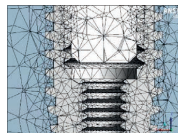
Fig. 2 - Reverse Engineering.
