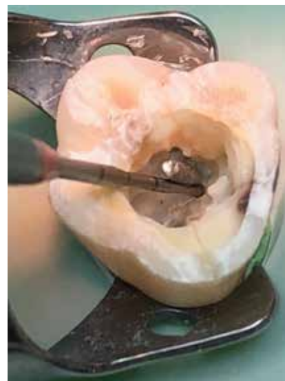
Fig. 7: Shaft-parallel cement-line dissection of a stainless-steel post with a Muncce Discovery Bur.
