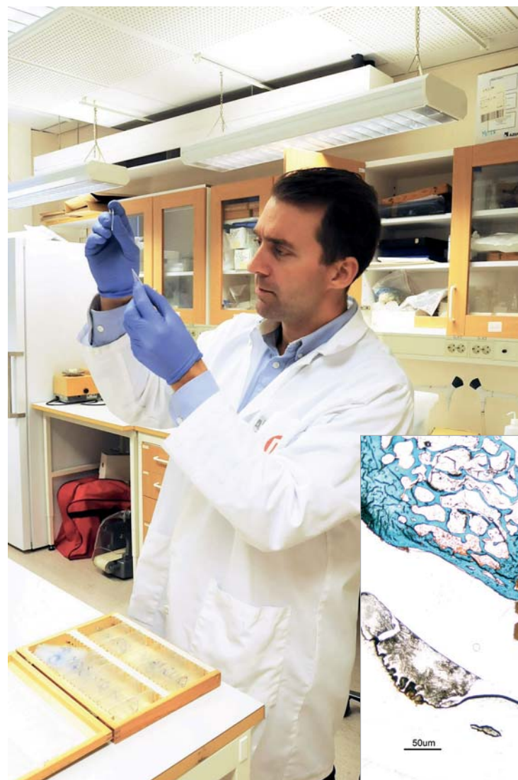
*Dr Johansson is examining histological sections of the implant in rabbit bone before looking at this in the microscope. This is a histological image from a PEEK implant with a hydroxyapatite coating. This one is implanted into rabbit bone and retrieved after three weeks of healing. At the bottom of the implant you can see the osteoconductive properties of hydroxyapatite on PEEK as the bone bends and grow along the implant surface.
