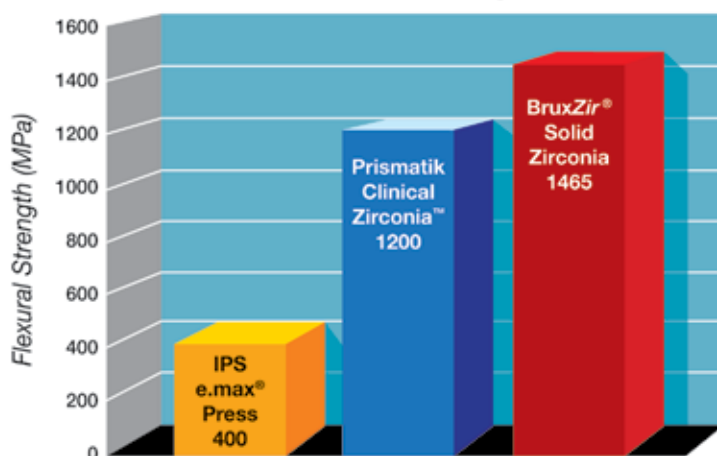
Flexural Strength 1
