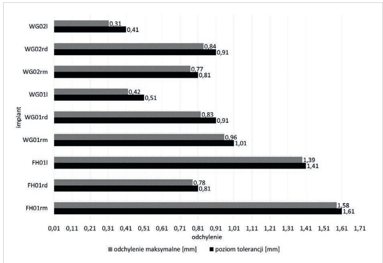
Fig. 4: Deviation levels for particular implants set with maximum point deviations. Implant naming: WG/FH, sample number, l/r, m/d (FH = freehand; WG = with guide; I = left; r = right; m = mesial; d = distal).
